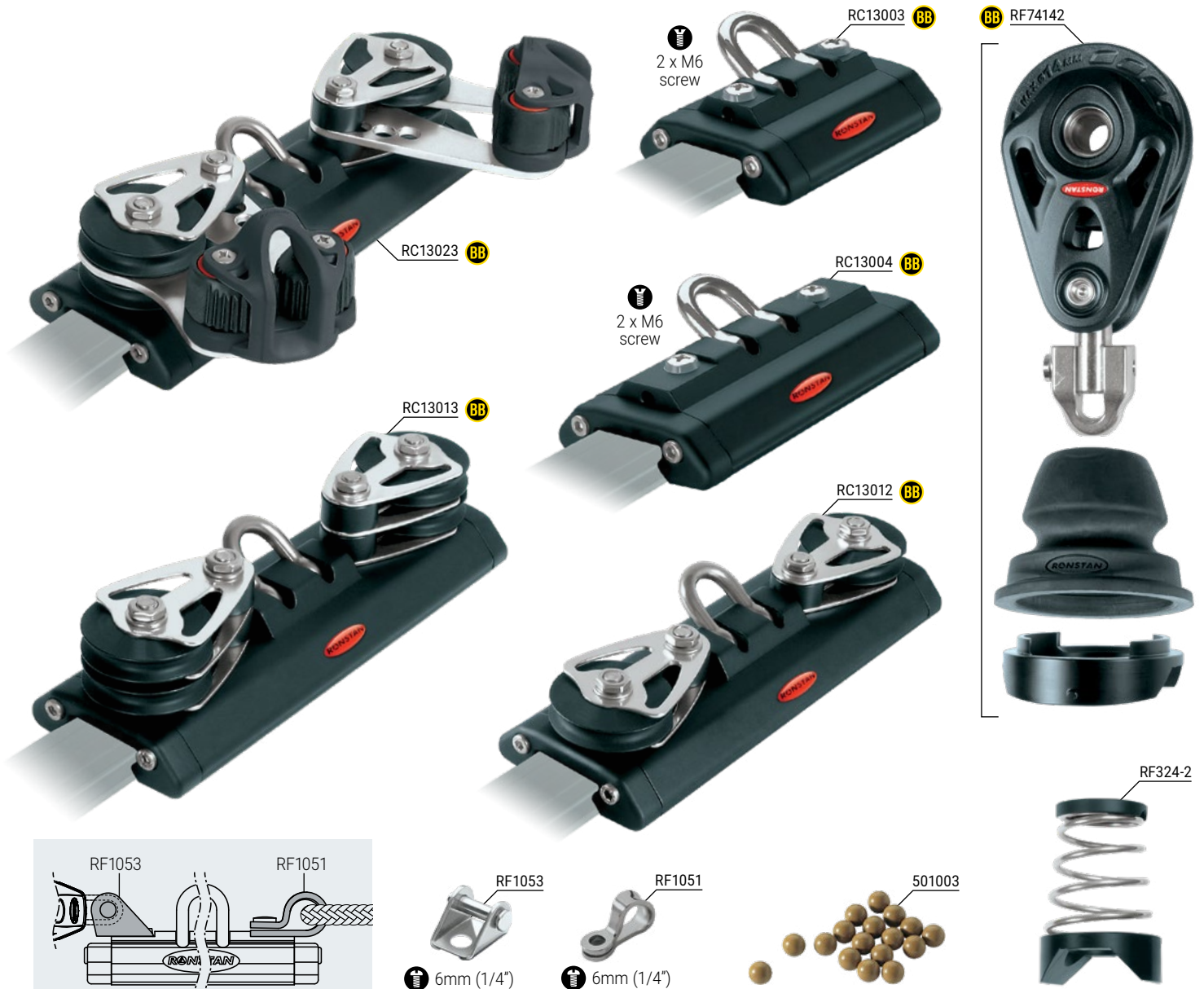
TYPICAL ADD-ON BECKET ARRANGEMENTS
