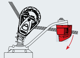
Cleat and wedge kit can be mounted on underside of arm for downward uncleating if preferred.
