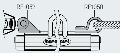
TYPICAL ADD-ON BECKET ARRANGEMENTS
