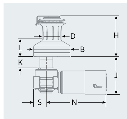
E1 electric motor conversion kits also available
